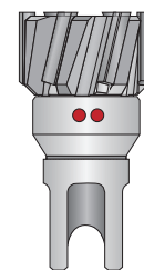
Right-Hand Helical Flute
