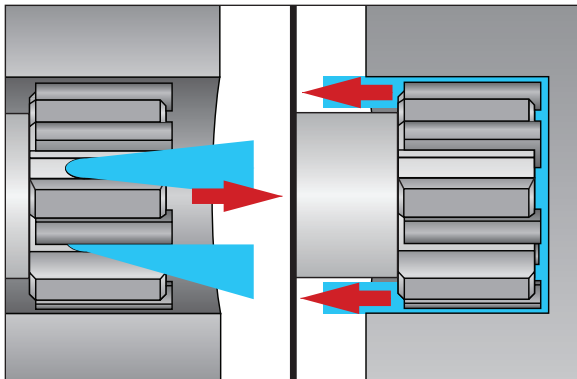
Straight Flute - Through or Blind Holes
